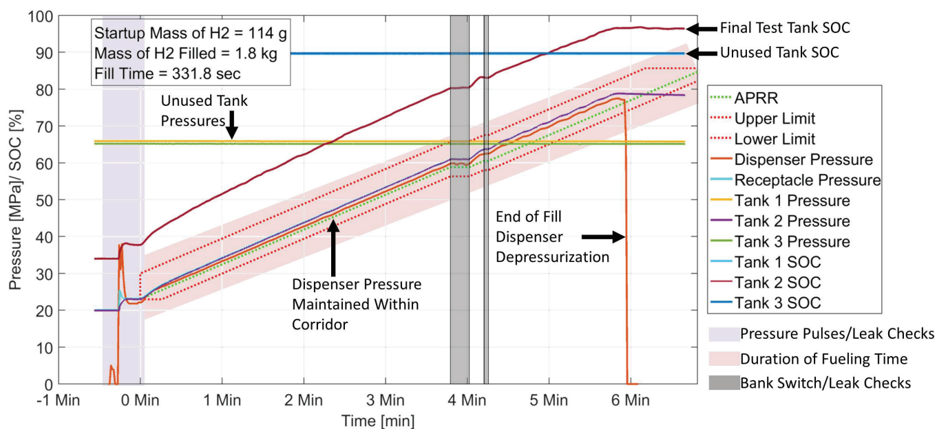
FIGURE 41: SAMPLE PASSING HySTEP PRESSURE DATA
