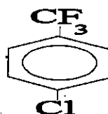
Figure VI-1 Structure of p-chlorobenzotrifluoride
