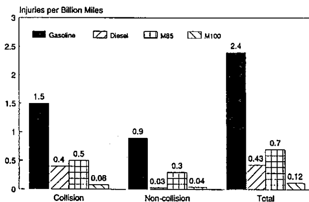
Figure 9 1986 LDV/LDT Fire Injury Comparison (Normalized) [1,2,3,6]
