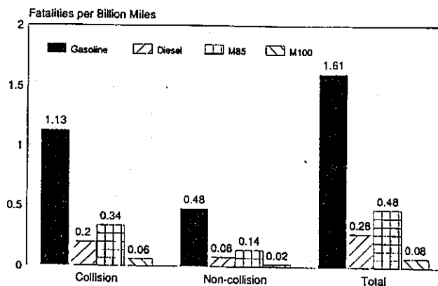
Figure 8 1986 HDV Fire Fatality Comparison (Normalized) [1,2,3,6]
