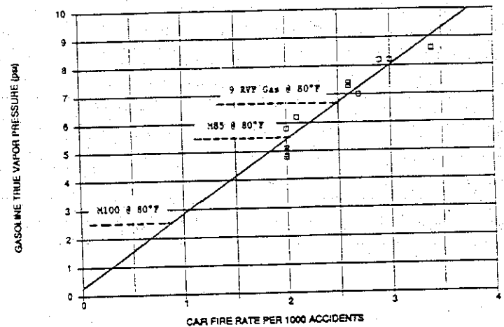
Figure 2 Effect of Fuel Volatility on the Car Fire Rate (3,8,9)
