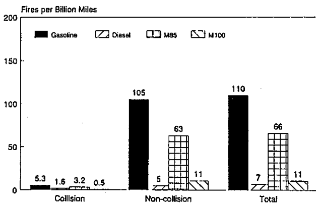
Figure 5 1986 LDV/LDT Fire Comparison (Normalized) [1,2,3,6]
