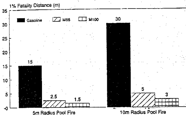
Figure 4 1% Fatality Distance From Fire's Edge [12]
