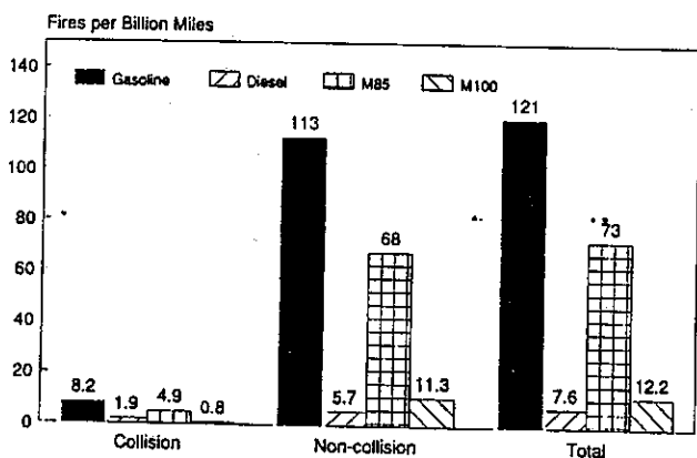
Figure 6 1986 HDV Fire Comparison (Normalized) [1,2,3,6]
