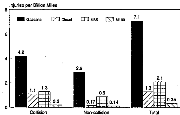
Figure 10 1986 HDV Fire Injury Comparison (Normalized) [1,2,3,6]
