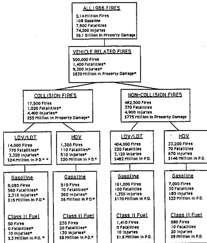
FIGURE 1 VEHICLE FIRE DISTRIBUTION (1,2)
