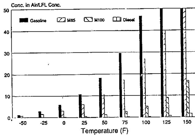
Figure 3 Flammability Index
