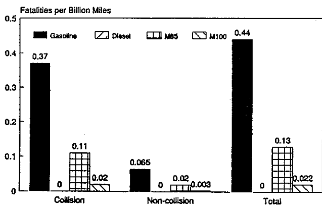
Figure 7 1986 LDV/LDT Fire Fatality Comparison (Normalized) [1,2,3,6]
