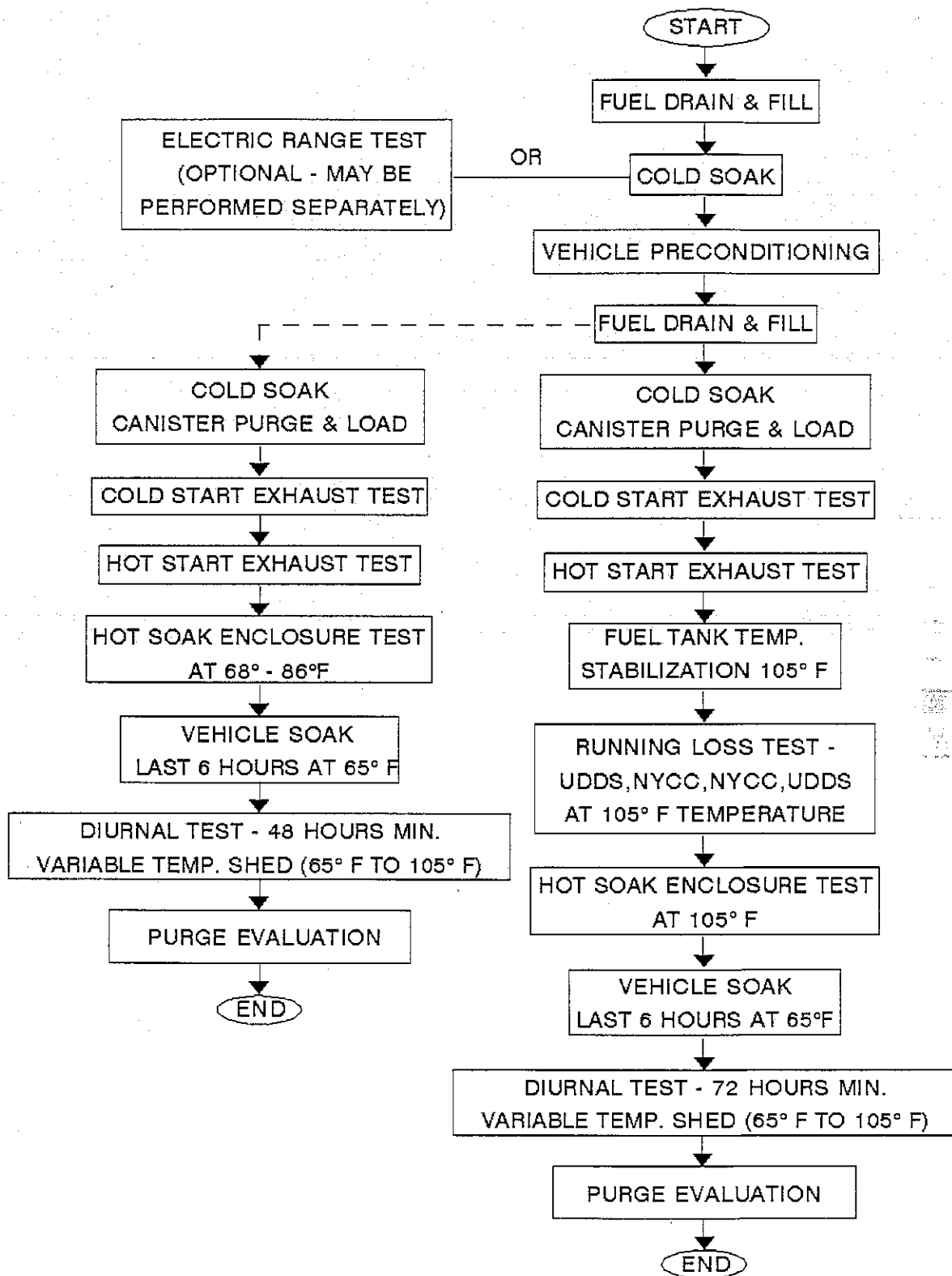
FIGURE 5. TEST PROCEDURES FOR 1996 AND SUBSEQUENT MODEL HYBRID ELECTRIC VEHICLES
