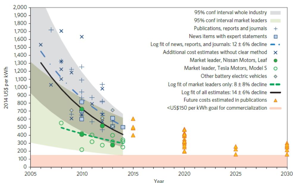
Figure 3: Cost of Lithium-ion Battery Packs in Light-Duty Battery Electric Vehicles
