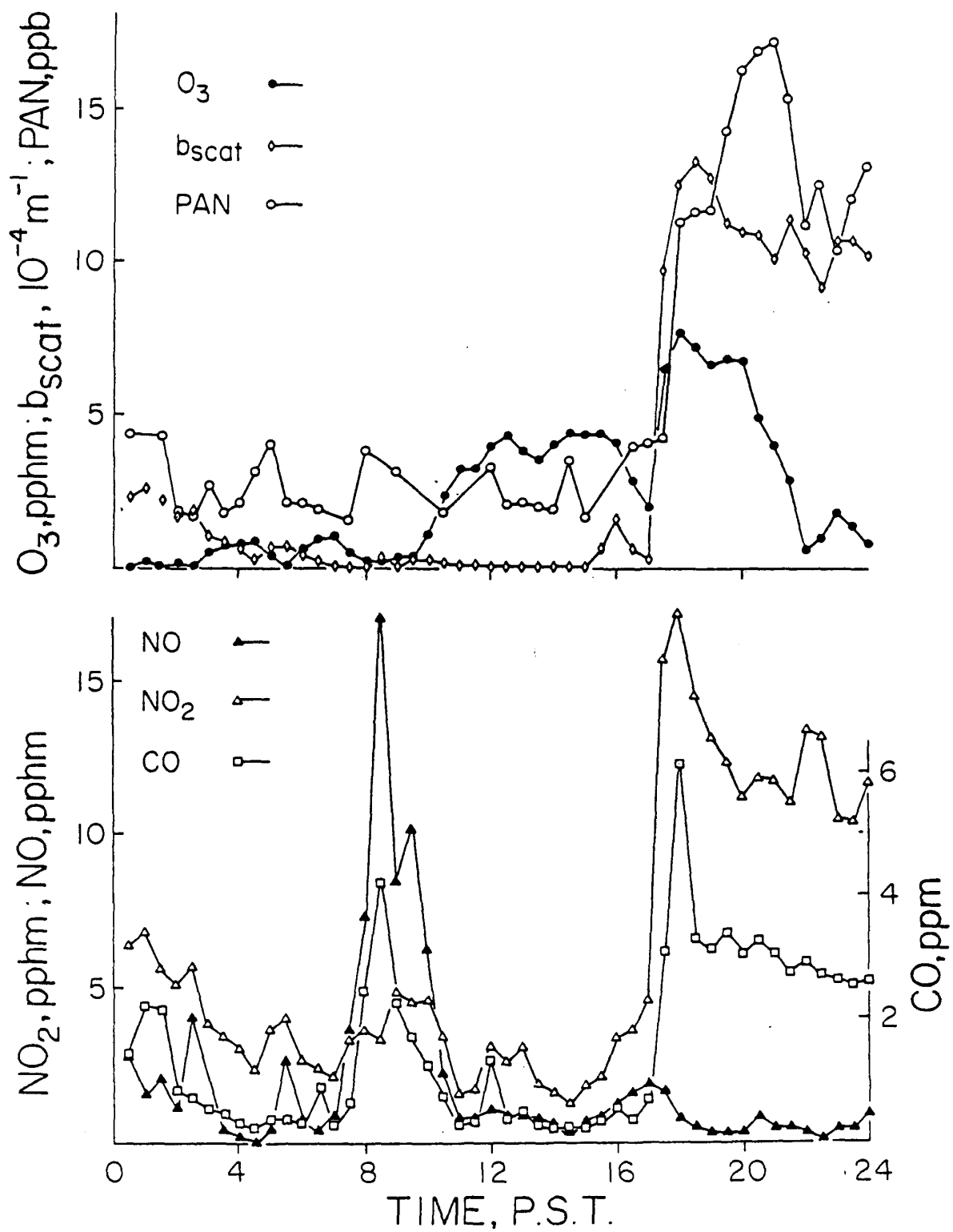
Diurnal profile for \text{NO} , \text{NO}_2 , \text{O}_3 , PAN, b_{\text{scat}} , and CO, February 16, 1977, Riverside, CA.
