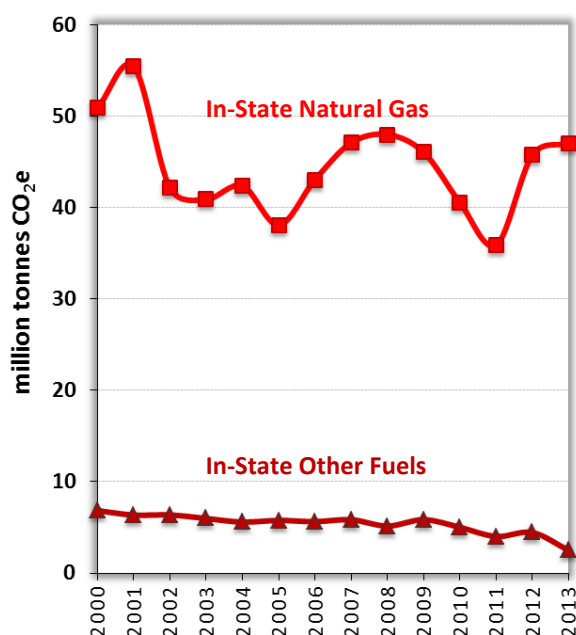
Figure 8. Electric Power Emissions (In-State)
